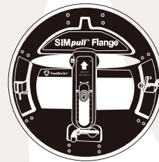
The SIMpull™ Flange 1 SIMpull™ Flange, 2 Electricians, 1 paralleled reel, Drill with 3/4 in. socket, Socket wrench (3/4 in.)
